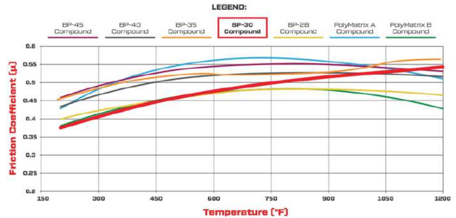
BP-30 Friction Coefficient and Temperature Values
